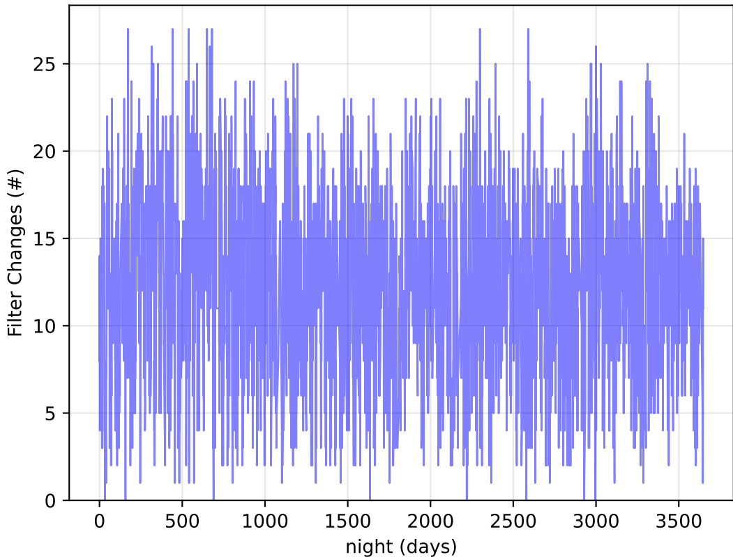
roll_pause_mjdp60_v3.4_10yrs : Filter Changes
