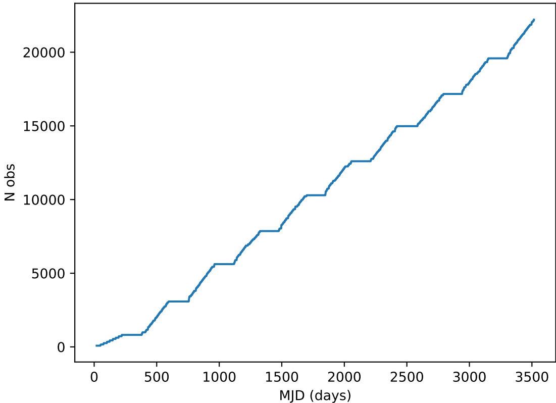
roll_pause_mjdp60_v3.4_10yrs note like DD:XMM_LSS%: Cumulative
