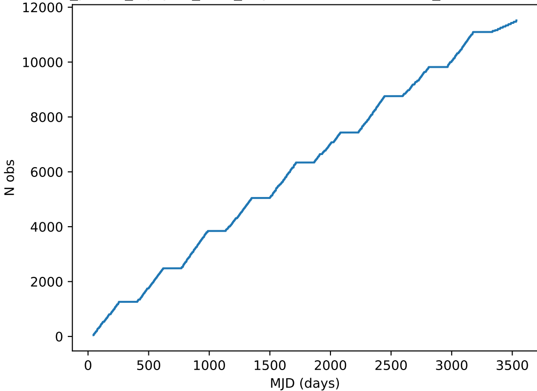
roll_pause_mjdp60_v3.4_10yrs note like DD:EDFS_a%: Cumulative
