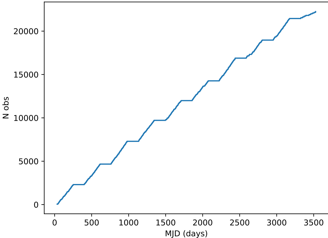
roll_pause_mjdp60_v3.4_10yrs note like DD:ECDFS%: Cumulative
