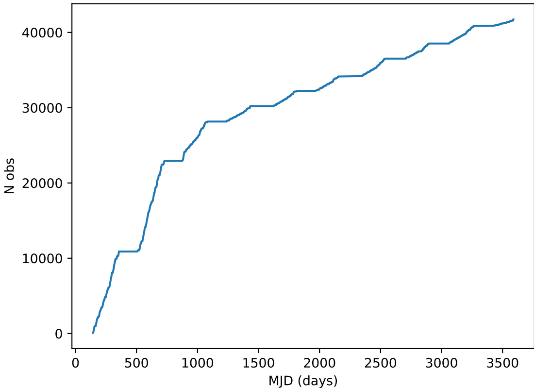
roll_pause_mjdp60_v3.4_10yrs note like DD:COSMOS%: Cumulative
