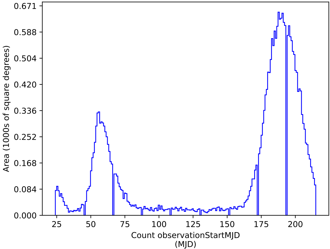
roll_pause_mjdp60_v3.4_10yrs i: Count observationStartMJD
