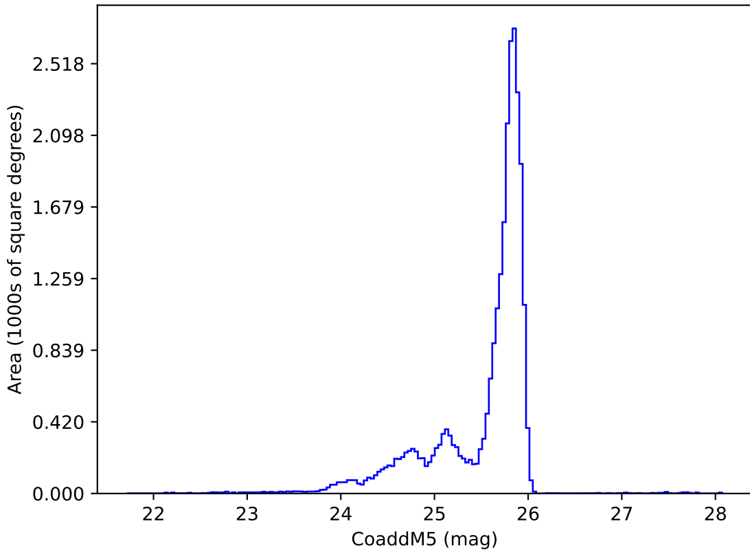
roll_pause_mjdp60_v3.4_10yrs z: CoaddM5
