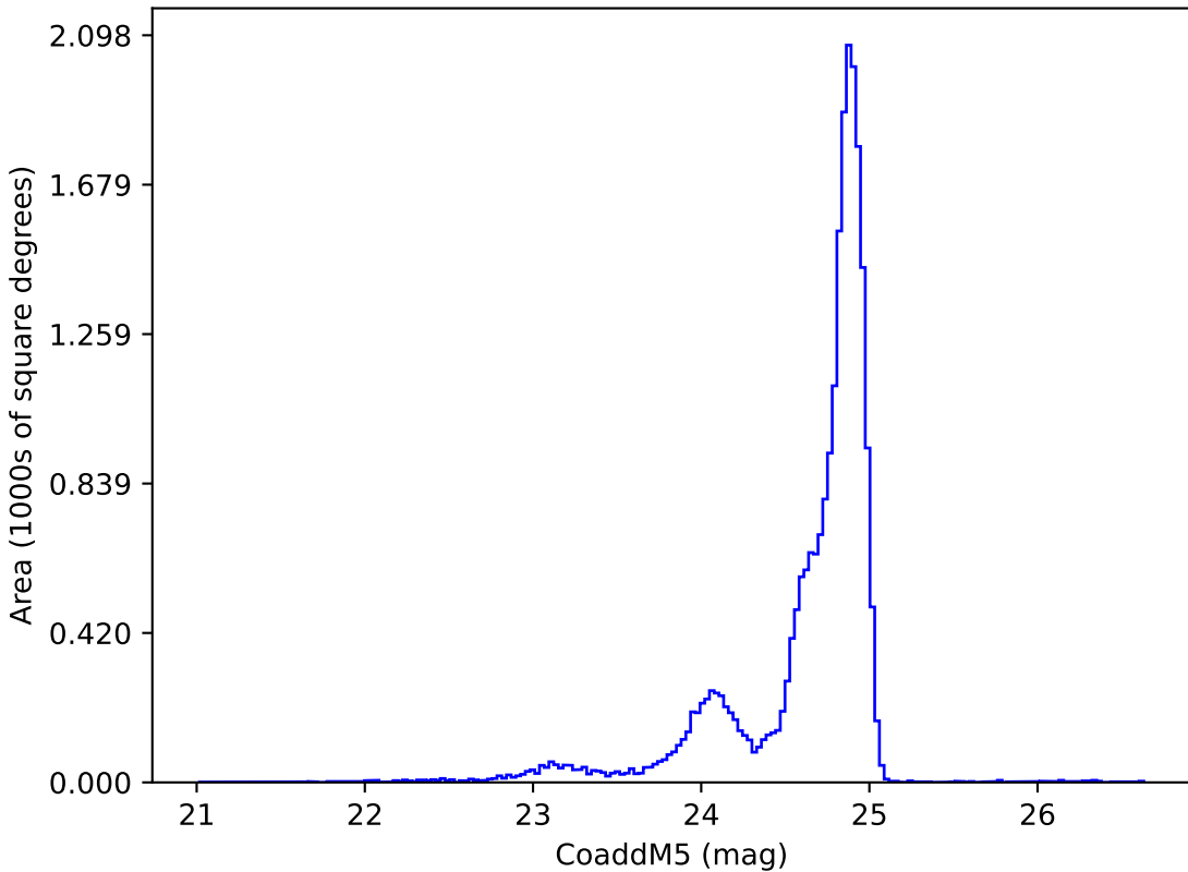
roll_pause_mjdp60_v3.4_10yrs y: CoaddM5
