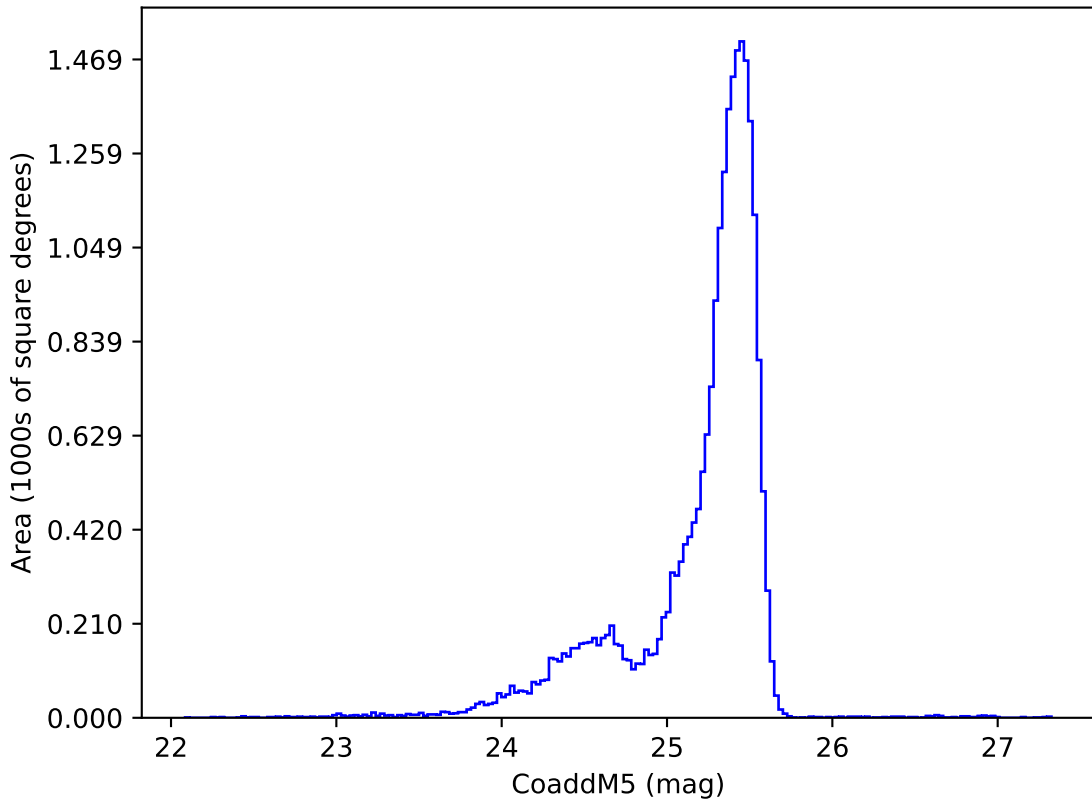
roll_pause_mjdp60_v3.4_10yrs u: CoaddM5
