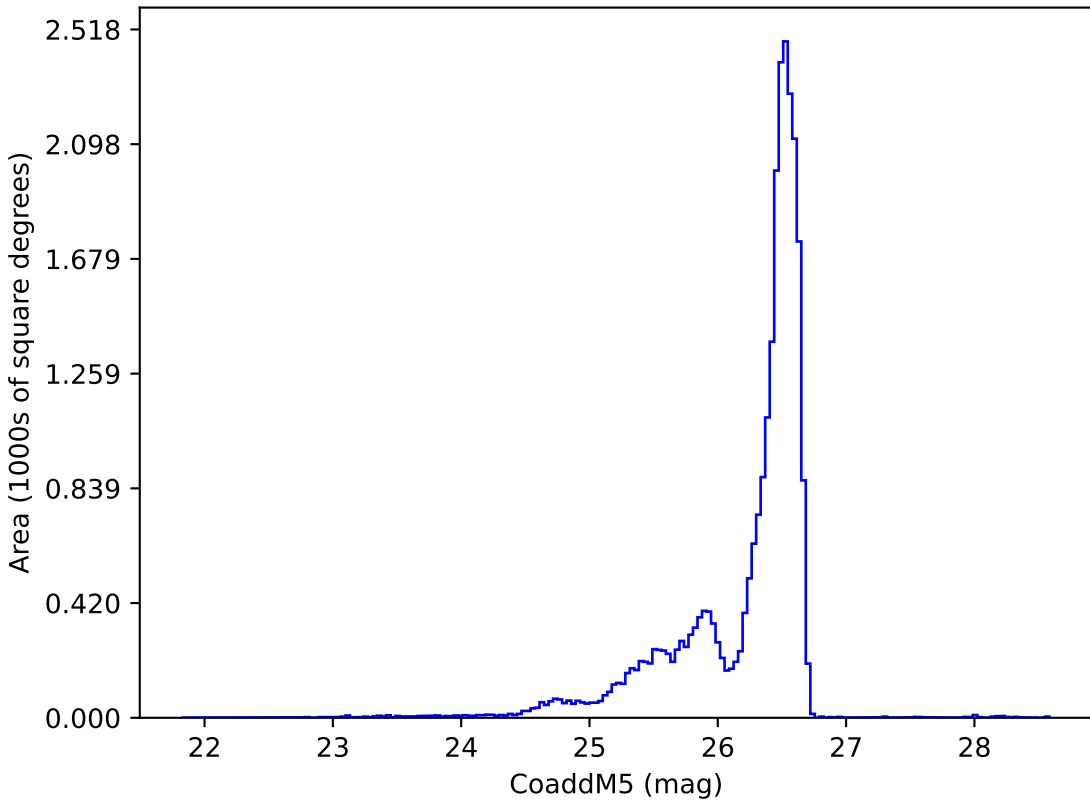
roll_pause_mjdp60_v3.4_10yrs i: CoaddM5
