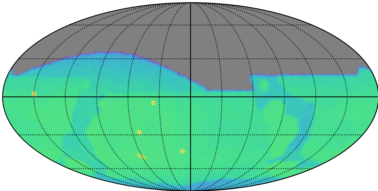
roll_pause_mjdp60_v3.4_10yrs g: CoaddM5
