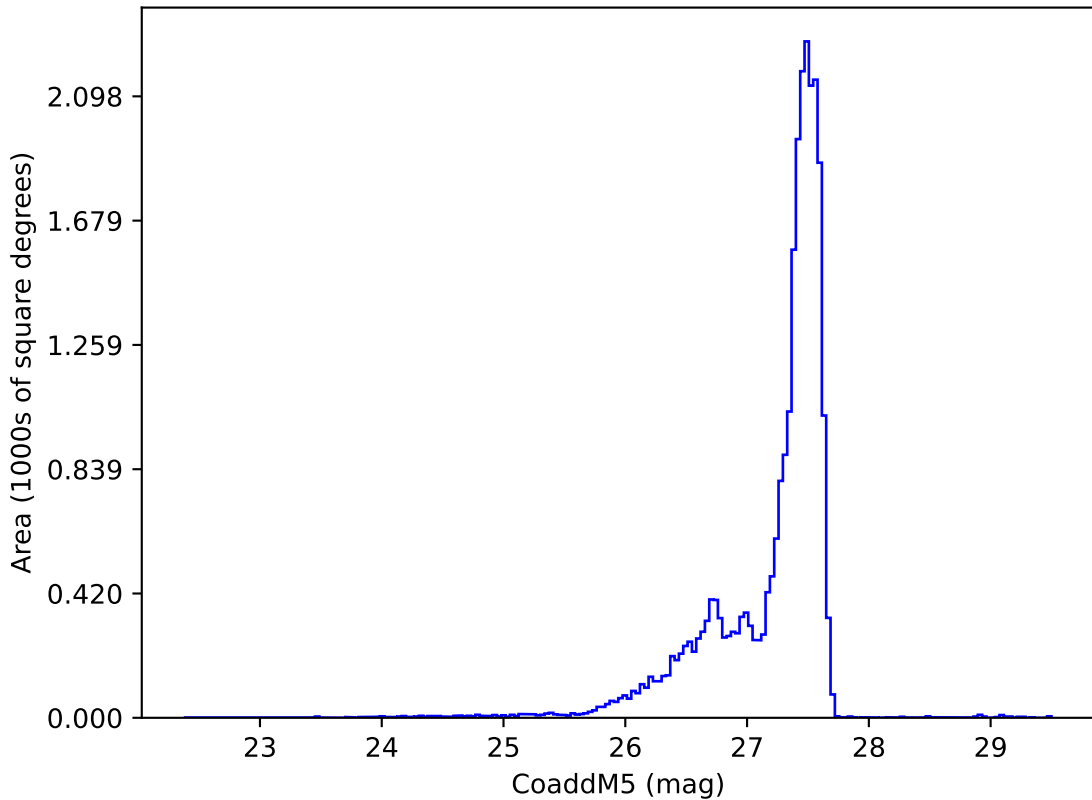
roll_pause_mjdp60_v3.4_10yrs : CoaddM5
