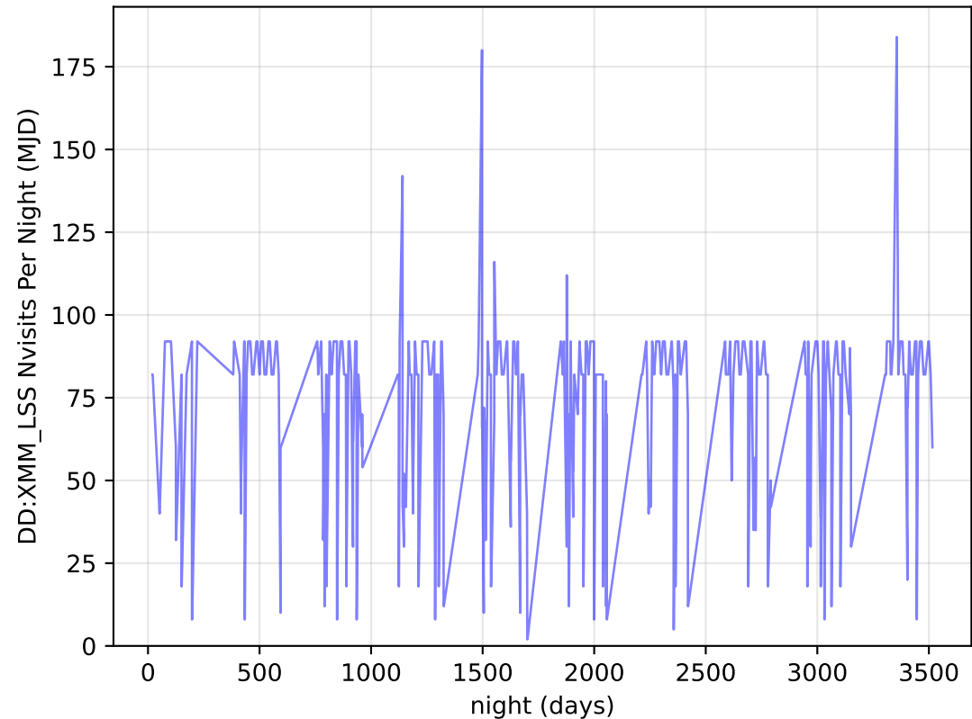
roll_pause_mjdp60_v3.4_10yrs all bands: DD:XMM_LSS Nvisits Per Night
