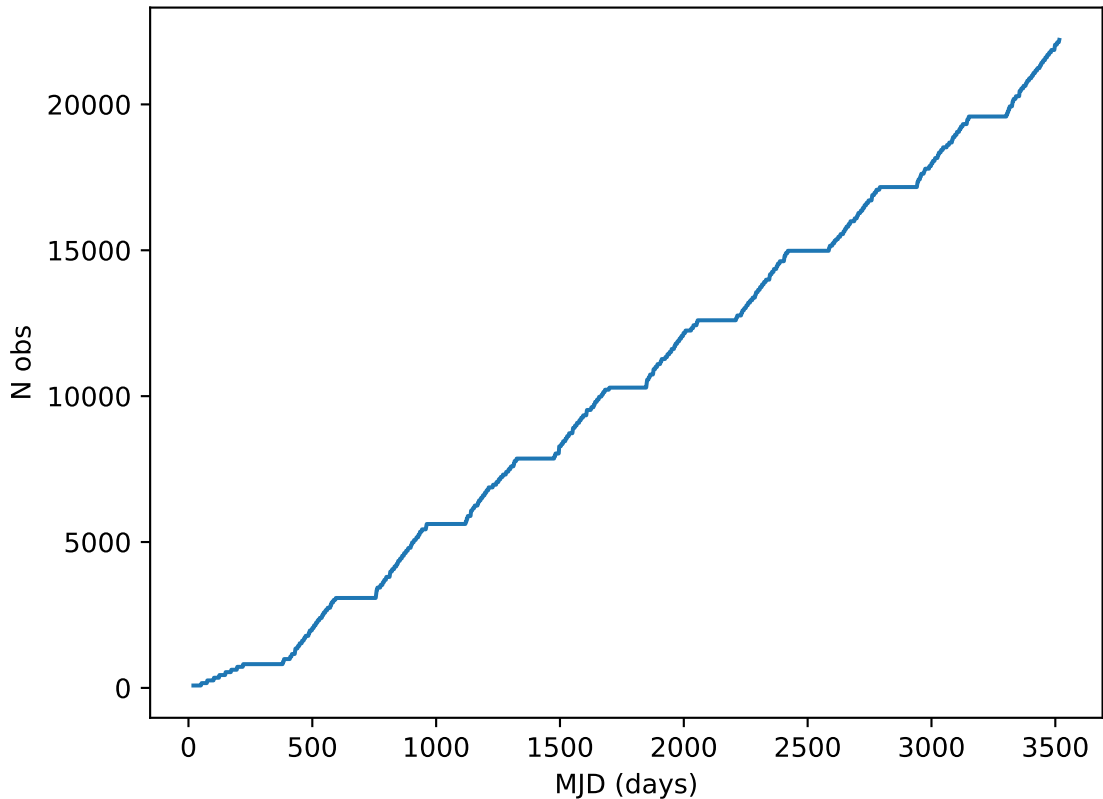
roll_pause_mjdp60_v3.4_10yrs all bands: DD:XMM_LSS Cumulative NVisits
