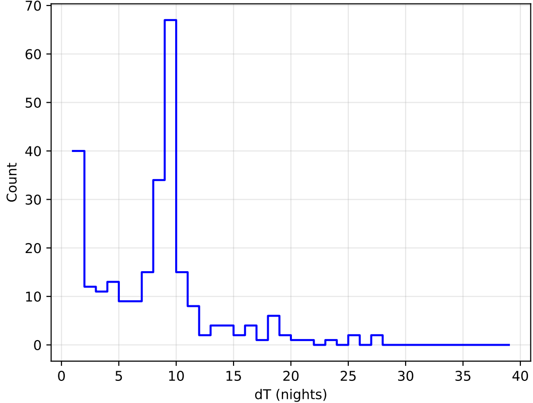
roll_pause_mjdp60_v3.4_10yrs all bands: DD:ELAISS1 Delta Nights Histogram
