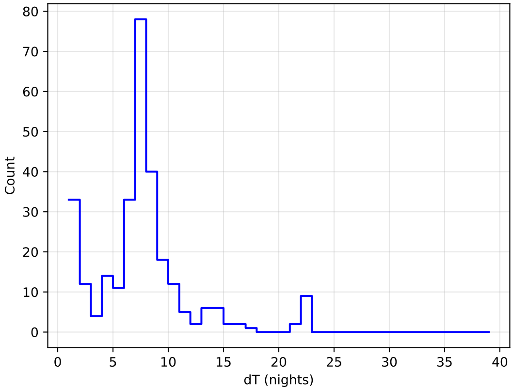
roll_pause_mjdp60_v3.4_10yrs all bands: DD:EDFS Delta Nights Histogram
