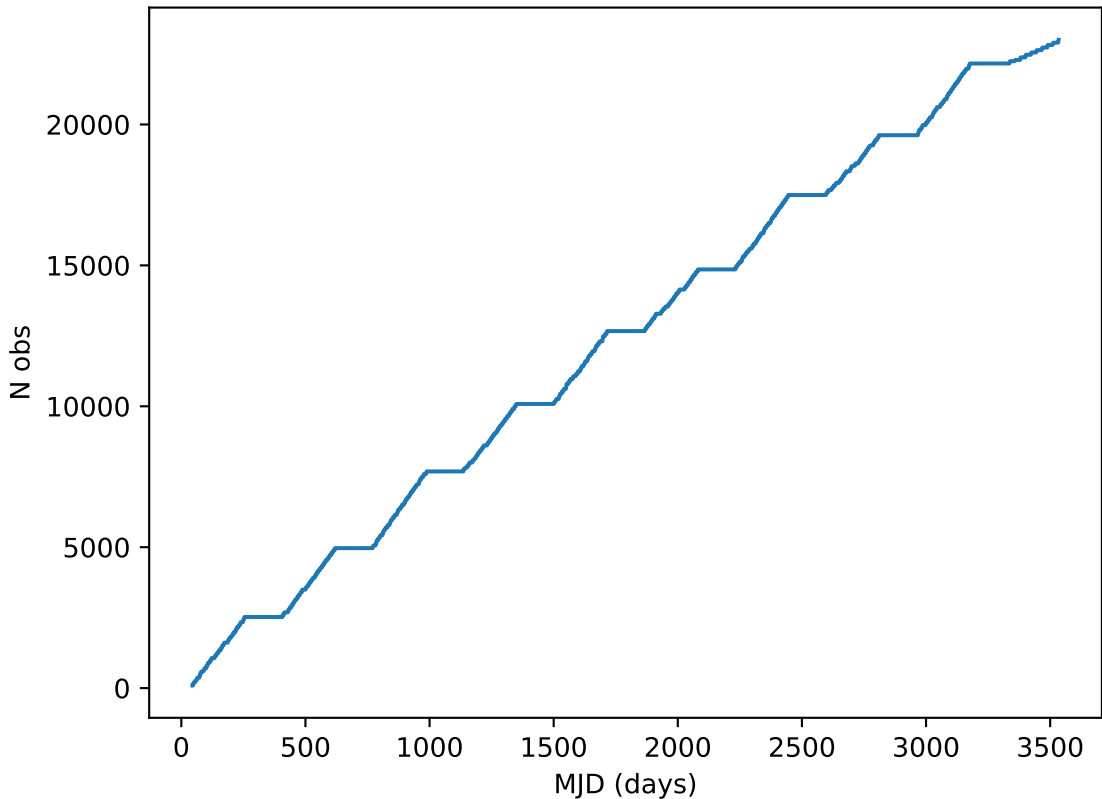
roll_pause_mjdp60_v3.4_10yrs all bands: DD:EDFS Cumulative NVisits
