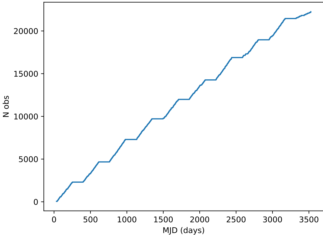
roll_pause_mjdp60_v3.4_10yrs all bands: DD:ECDFS Cumulative NVisits
