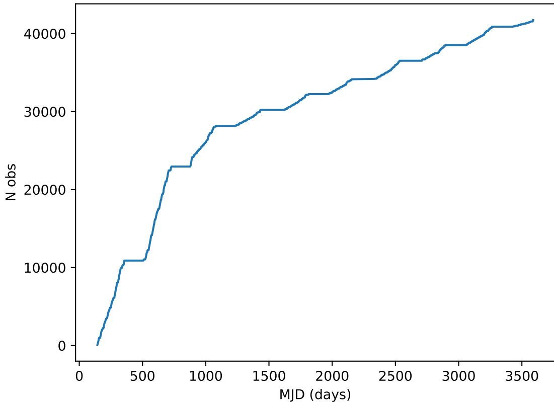
roll_pause_mjdp60_v3.4_10yrs all bands: DD: COSMOS Cumulative NVisits
