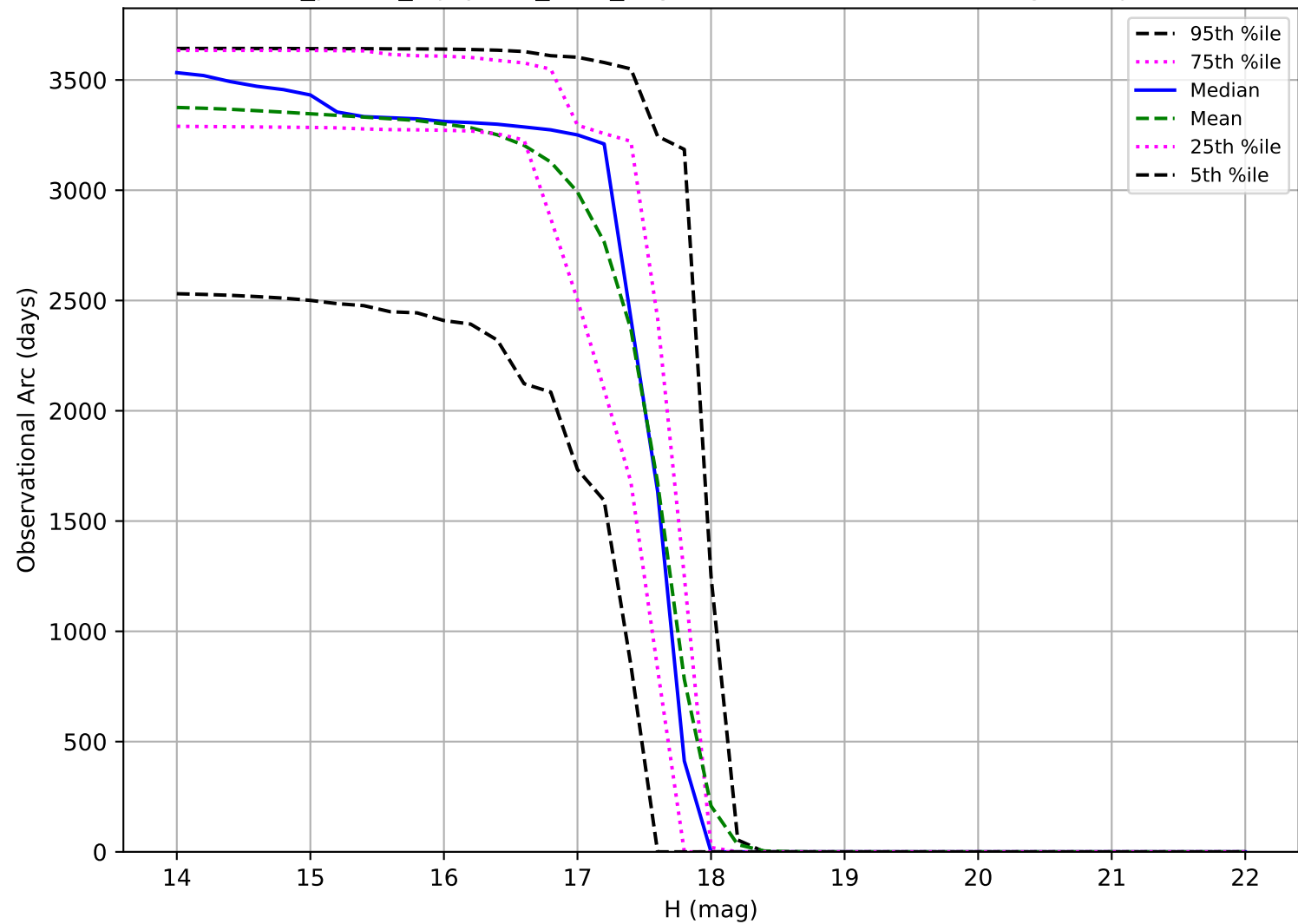
roll_pause_mjdp365_v3.4_10yrs: Observational Arc Length Trojan
