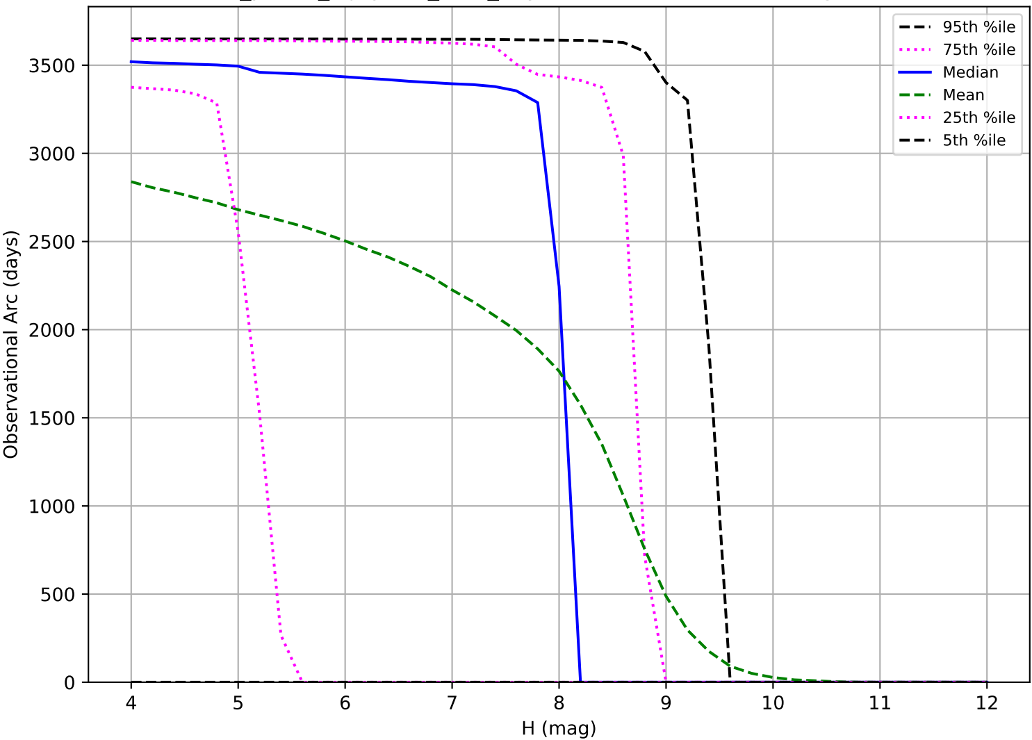
roll_pause_mjdp365_v3.4_10yrs: Observational Arc Length TNO
