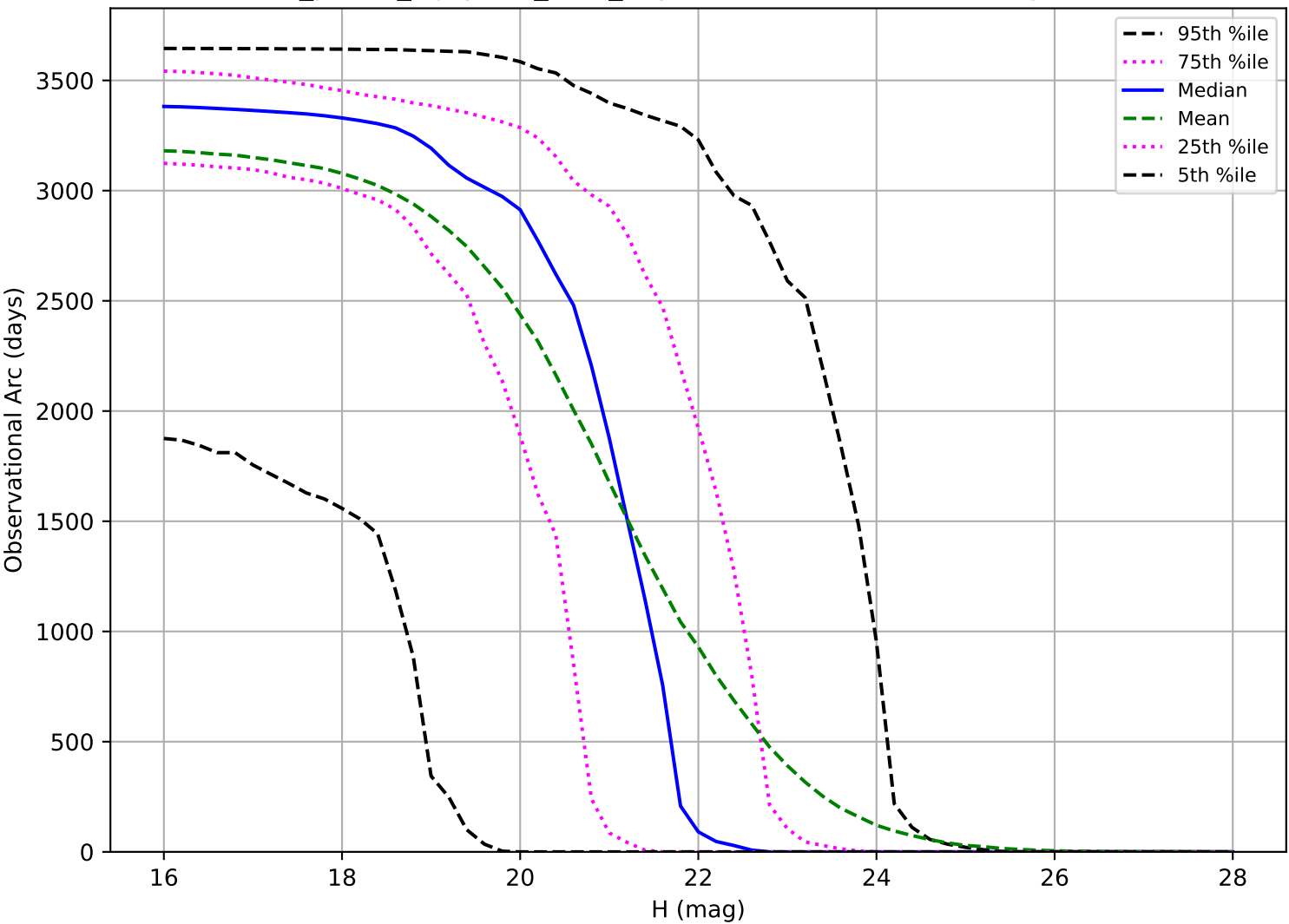
roll_pause_mjdp365_v3.4_10yrs: Observational Arc Length NEO
