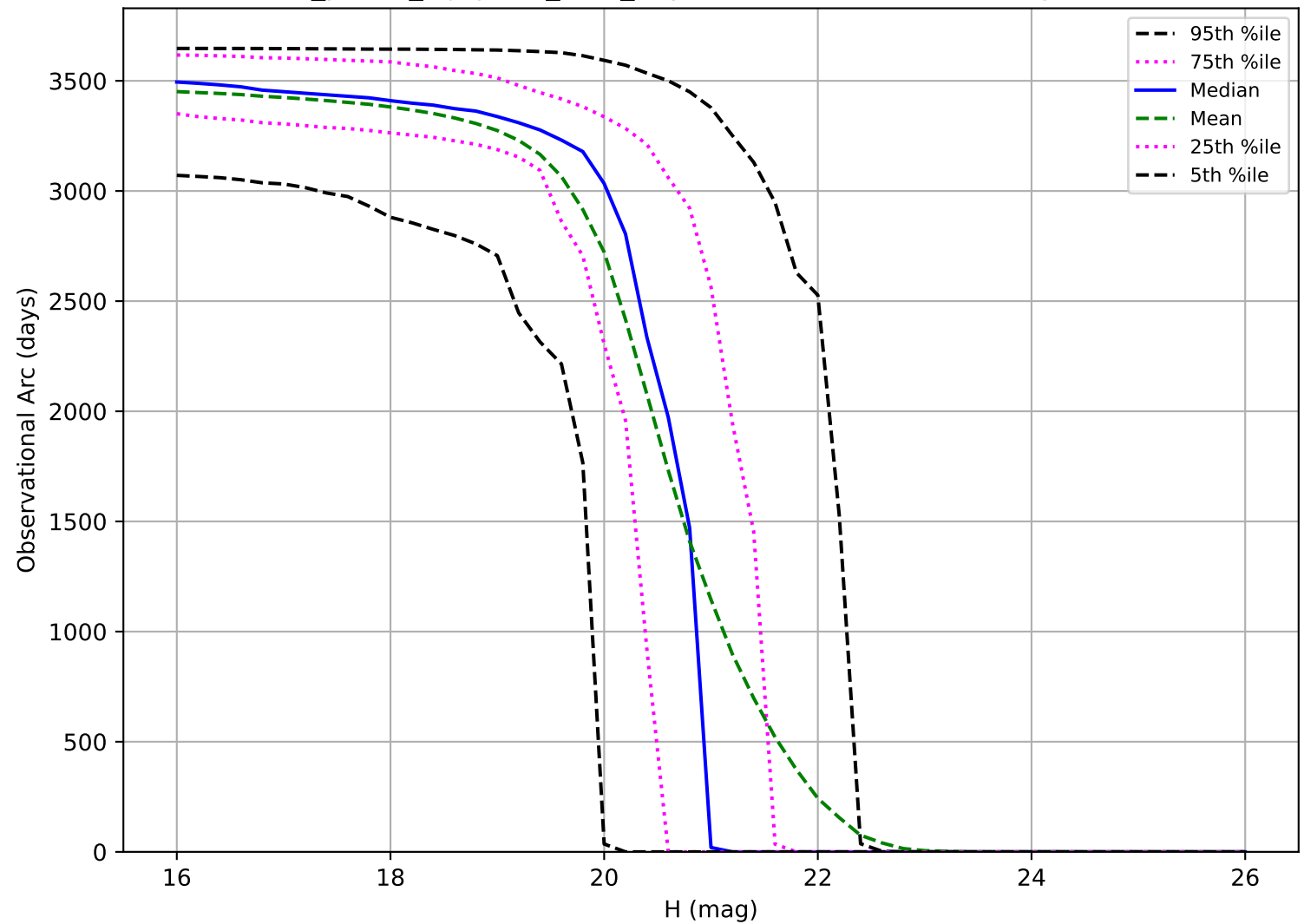
roll_pause_mjdp365_v3.4_10yrs: Observational Arc Length MBA
