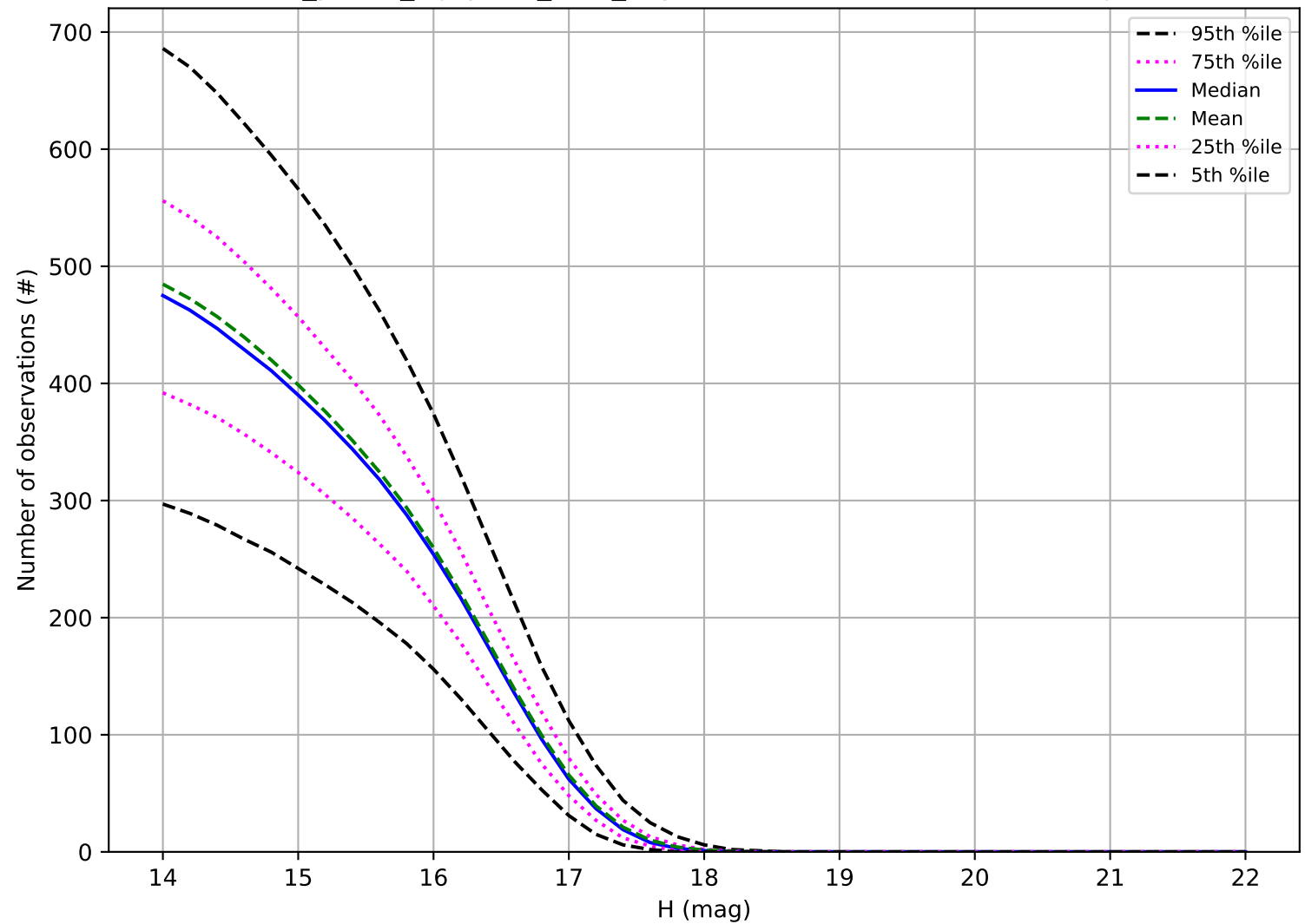
roll_pause_mjdp365_v3.4_10yrs: Number of observations Trojan
