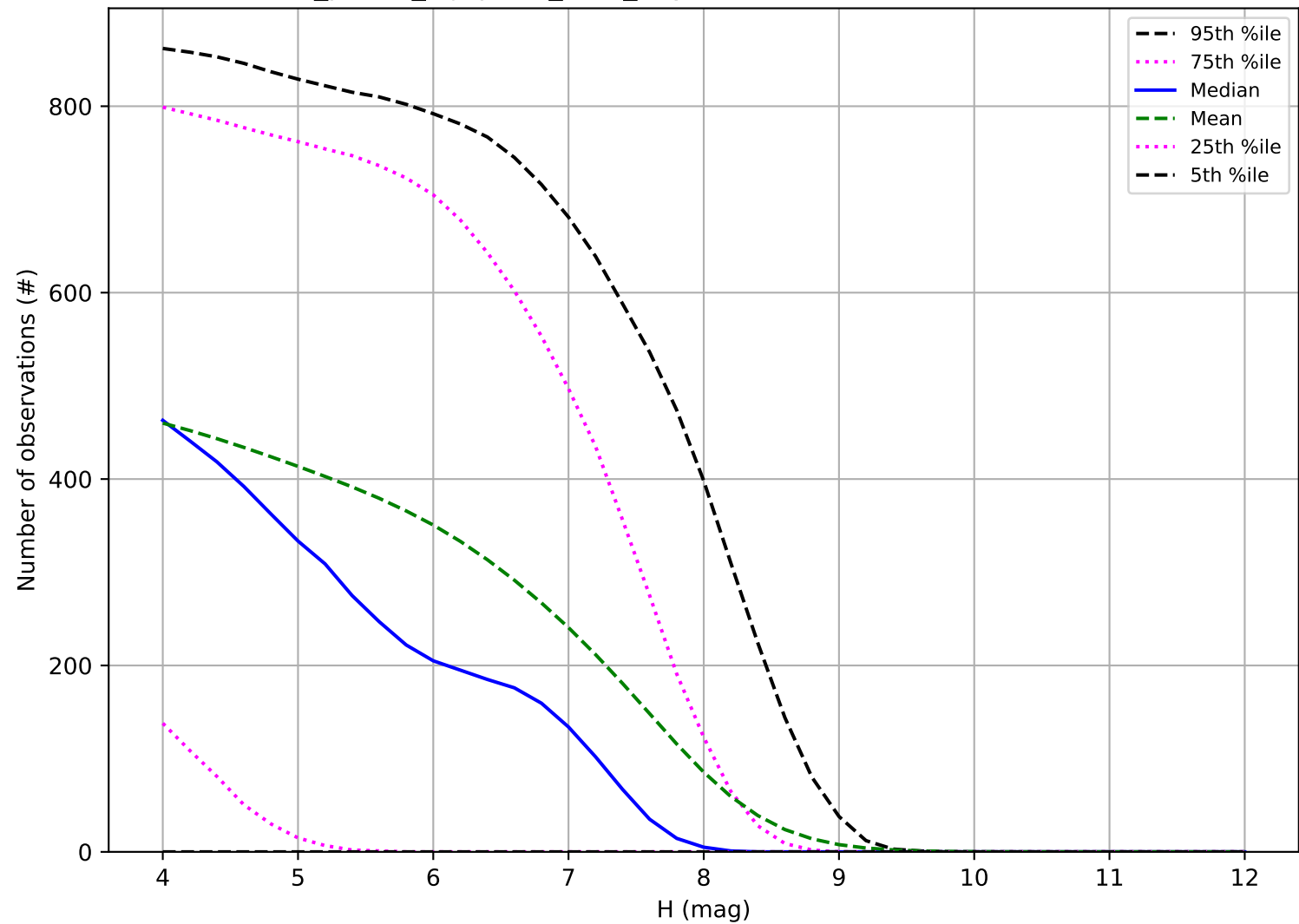
roll_pause_mjdp365_v3.4_10yrs: Number of observations TNO
