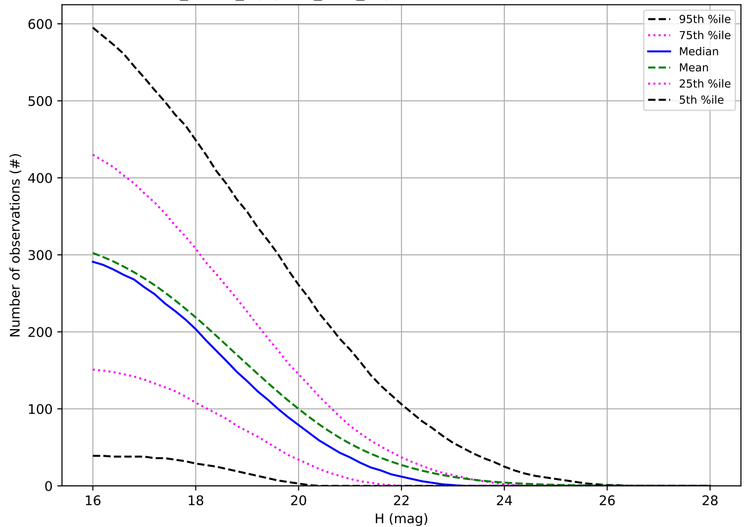
roll_pause_mjdp365_v3.4_10yrs: Number of observations PHA
