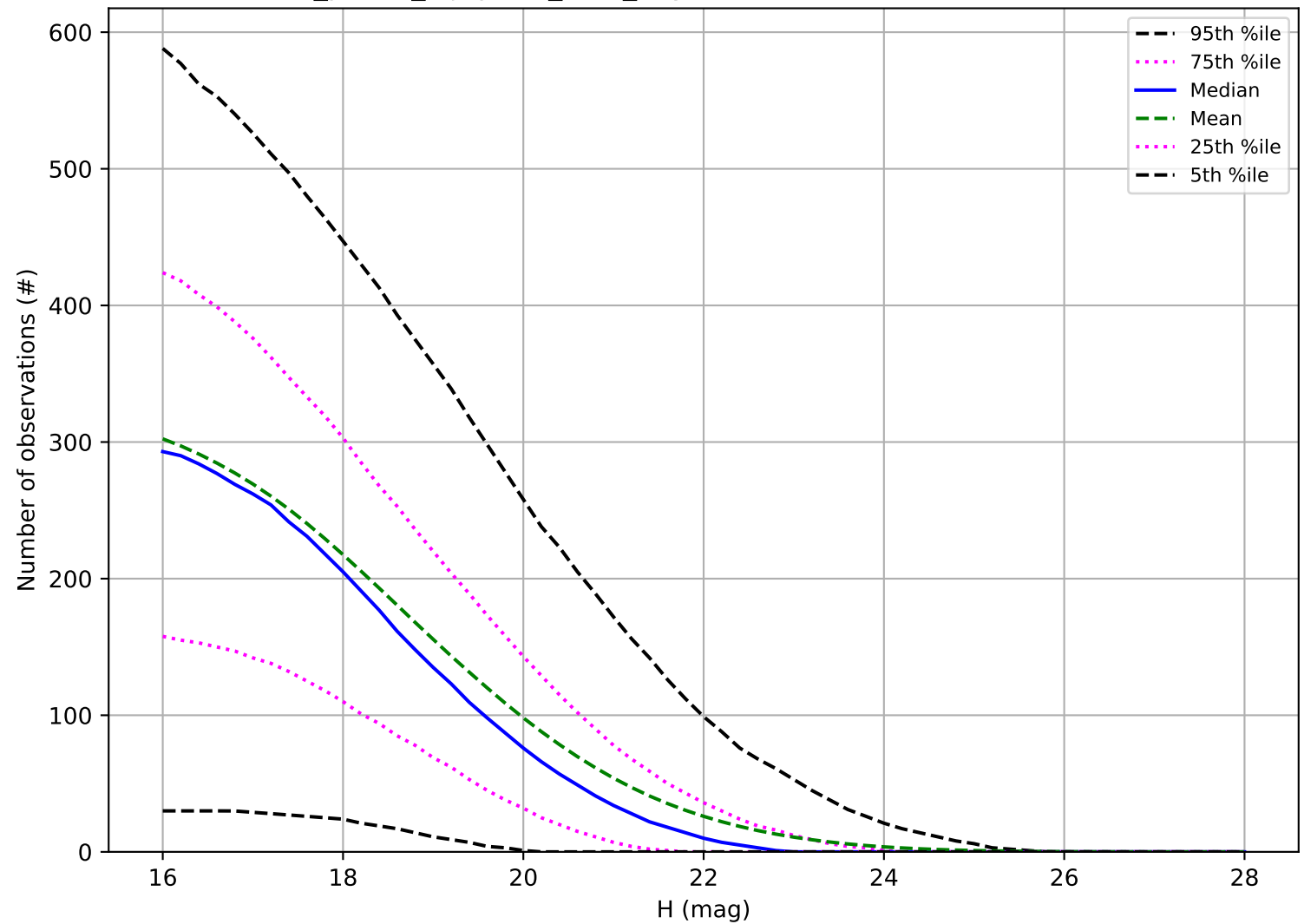
roll_pause_mjdp365_v3.4_10yrs: Number of observations NEO
