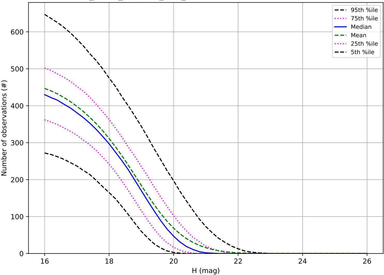
roll_pause_mjdp365_v3.4_10yrs: Number of observations MBA
