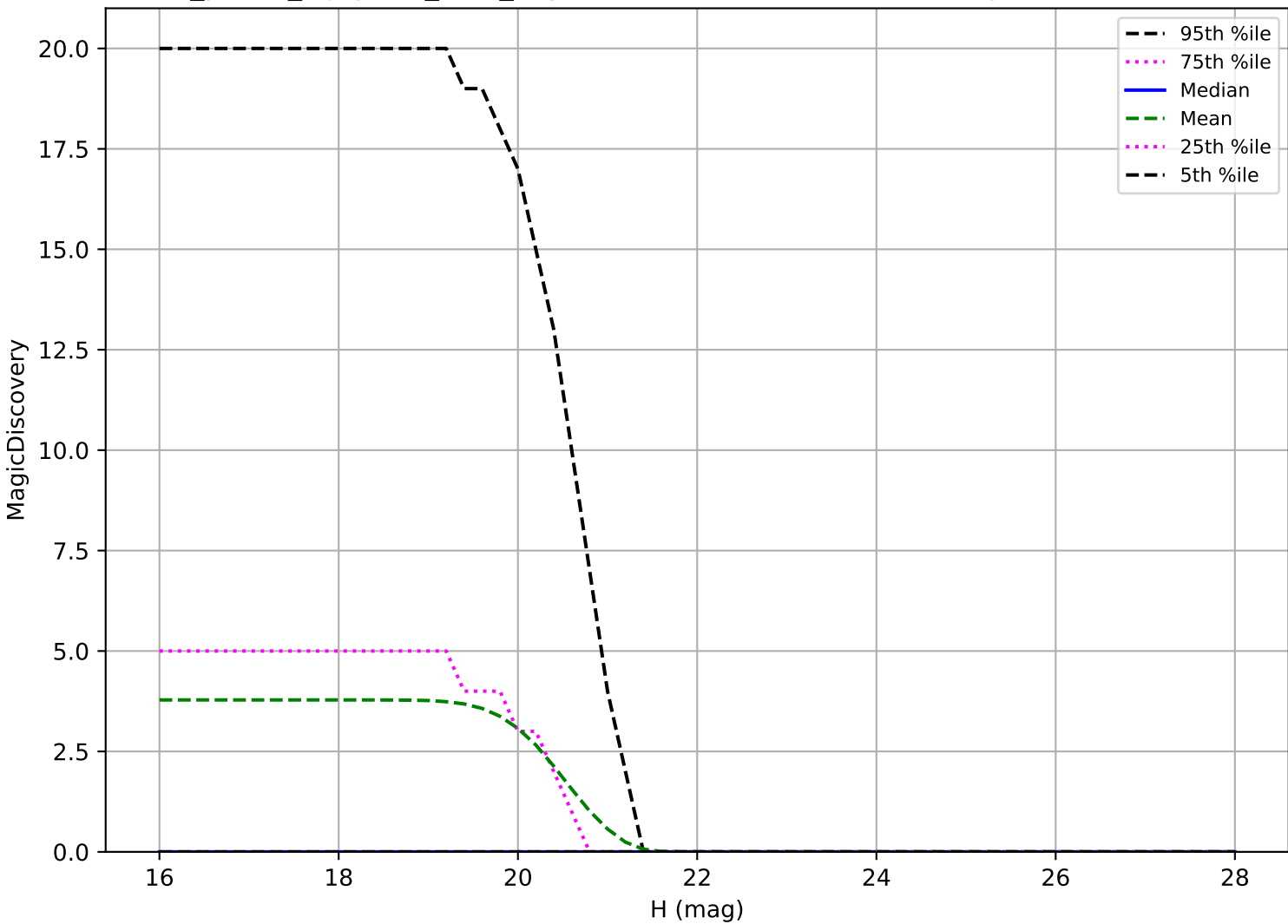
roll_pause_mjdp365_v3.4_10yrs: Vatira 6 detections in 60 nights detection loss
