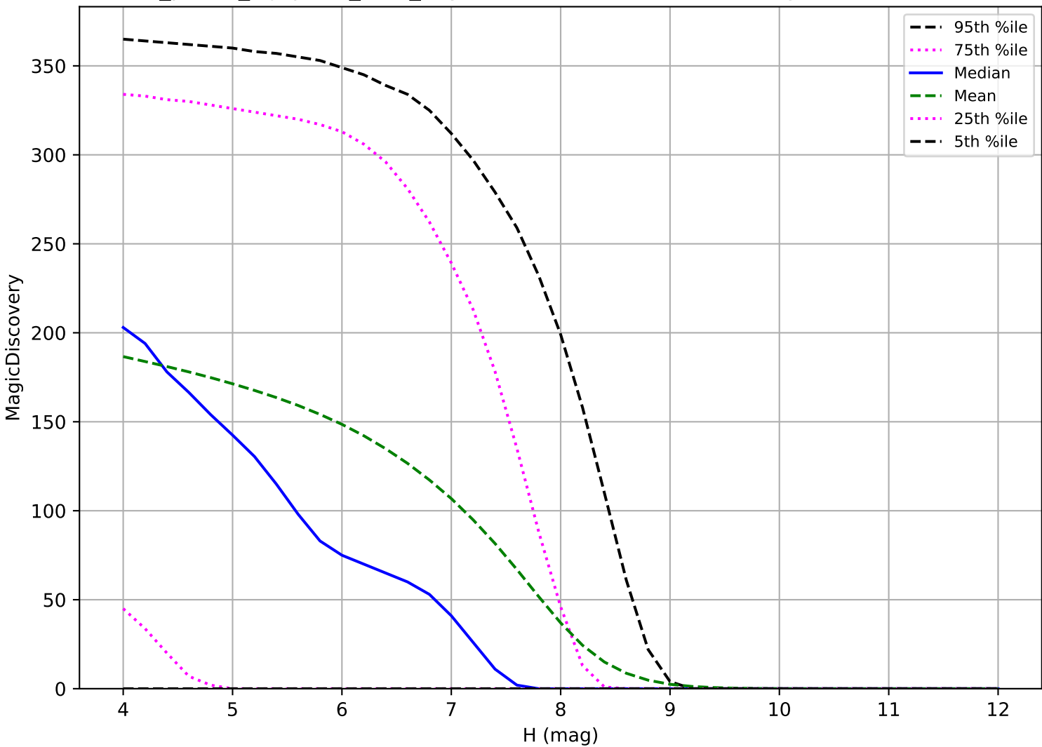
roll_pause_mjdp365_v3.4_10yrs: TNO 6 detections in 60 nights detection loss
