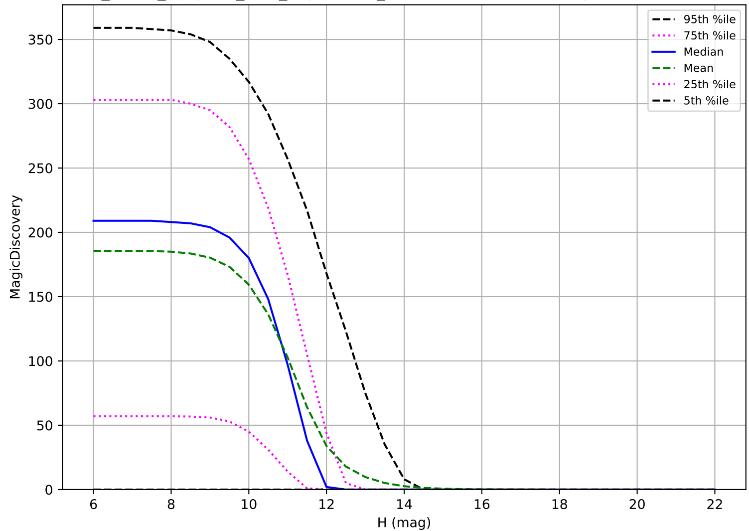
roll_pause_mjdp365_v3.4_10yrs: OCC_r20 6 detections in 60 nights detection loss
