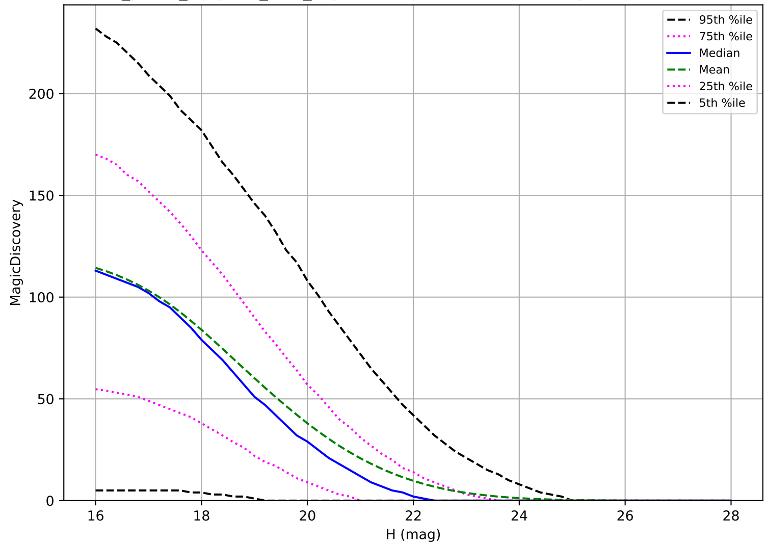
roll_pause_mjdp365_v3.4_10yrs: NEO 6 detections in 60 nights detection loss
