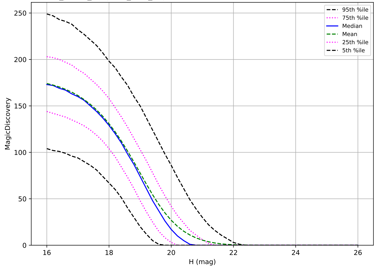
roll_pause_mjdp365_v3.4_10yrs: MBA 6 detections in 60 nights detection loss
