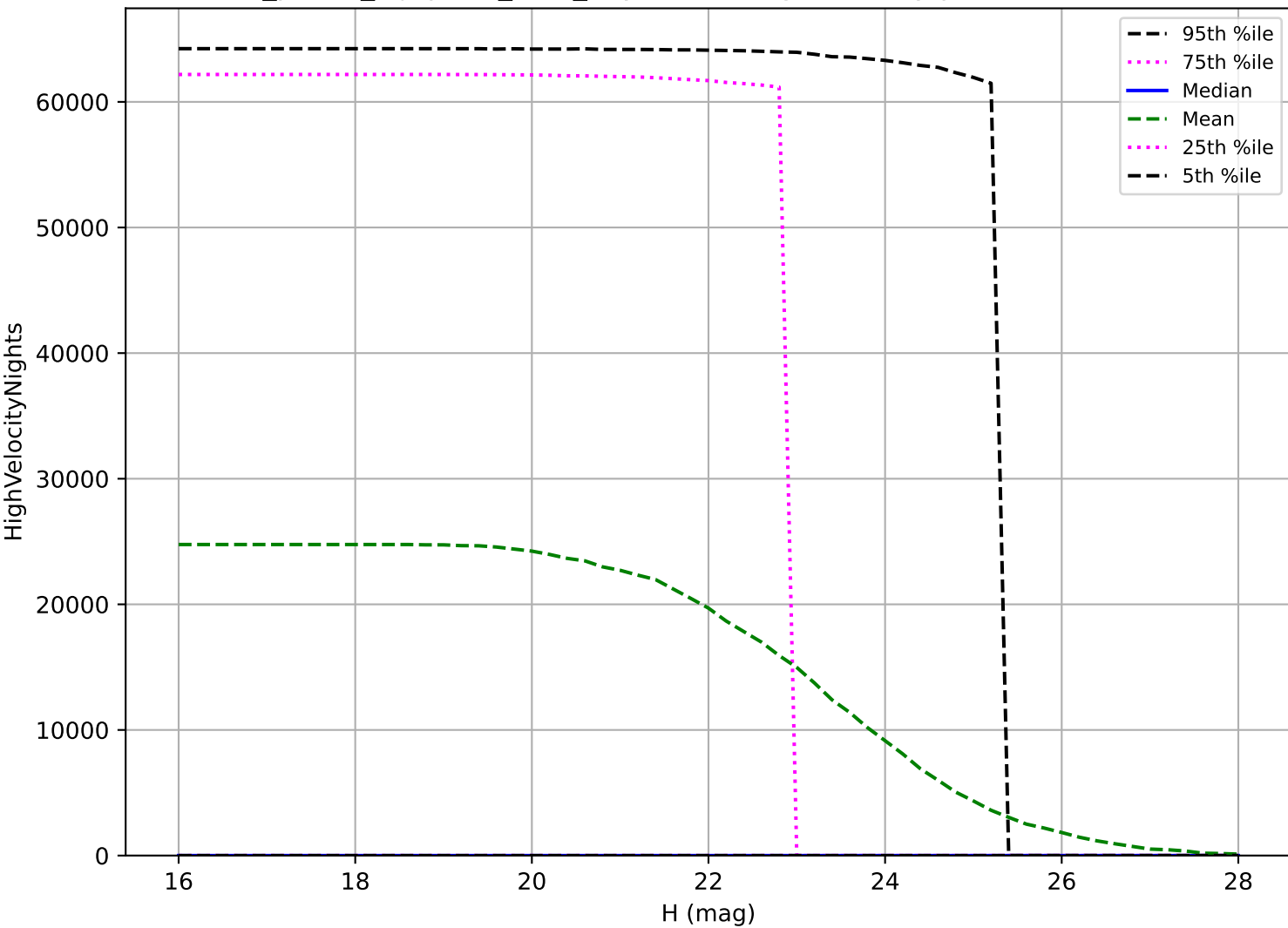
roll_pause_mjdp365_v3.4_10yrs: PHA High velocity pair detection loss
