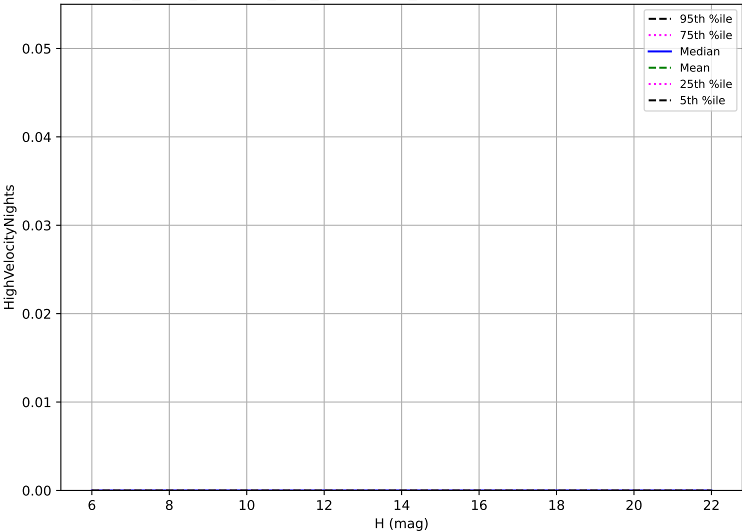
roll_pause_mjdp365_v3.4_10yrs: OCC_r5 High velocity pair detection loss
