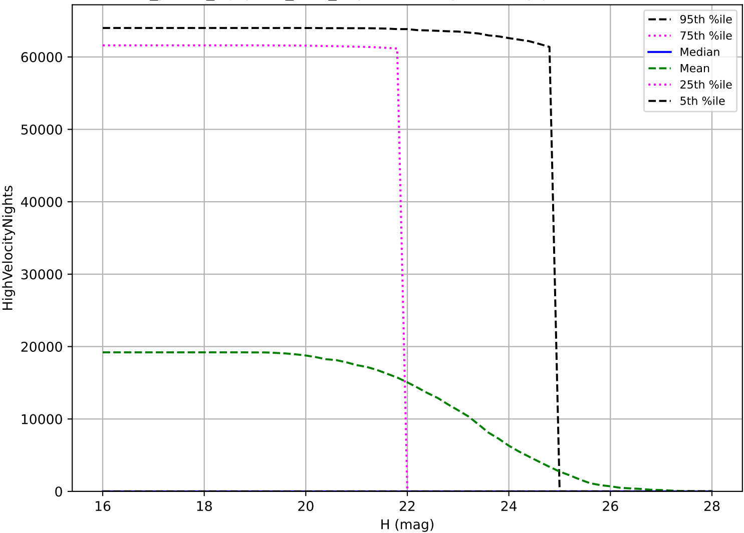
roll_pause_mjdp365_v3.4_10yrs: NEO High velocity pair detection loss
