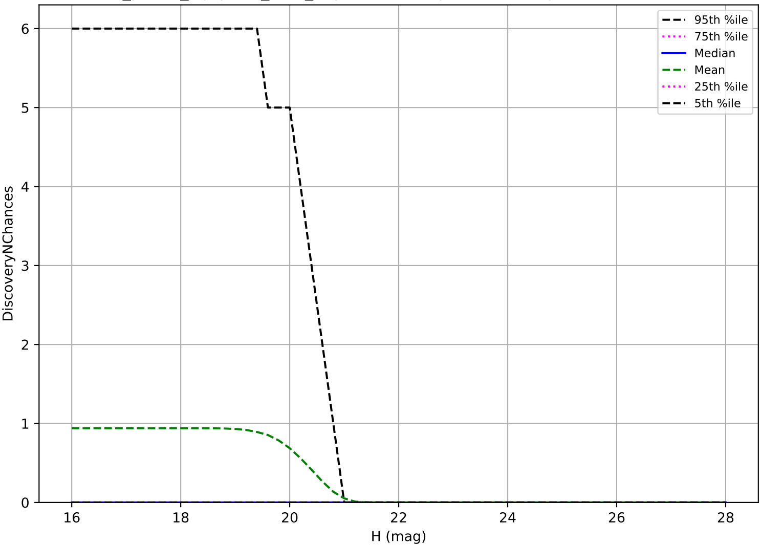
roll_pause_mjdp365_v3.4_10yrs: Vatira 3 pairs in 15 nights detection loss
