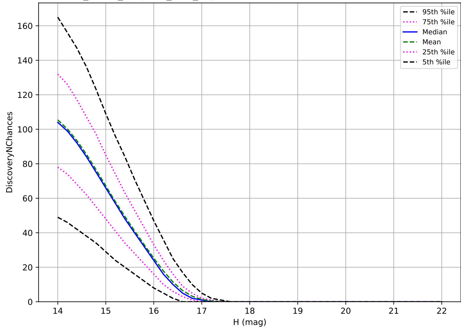
roll_pause_mjdp365_v3.4_10yrs: Trojan 3 pairs in 15 nights detection loss
