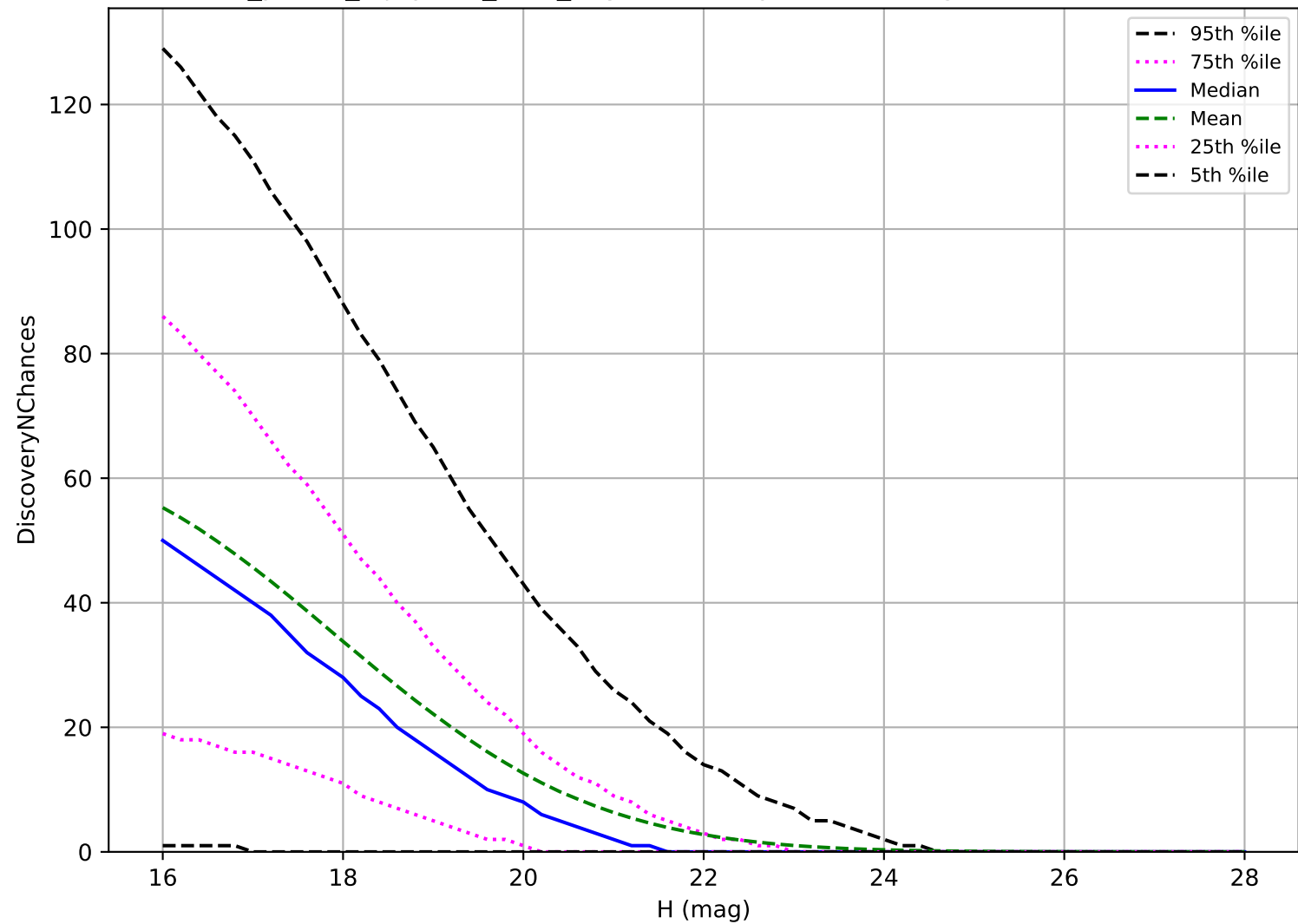
roll_pause_mjdp365_v3.4_10yrs: PHA 3 pairs in 15 nights detection loss
