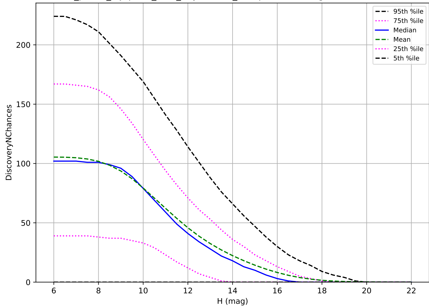
roll_pause_mjdp365_v3.4_10yrs: OCC_r5 3 pairs in 15 nights detection loss
