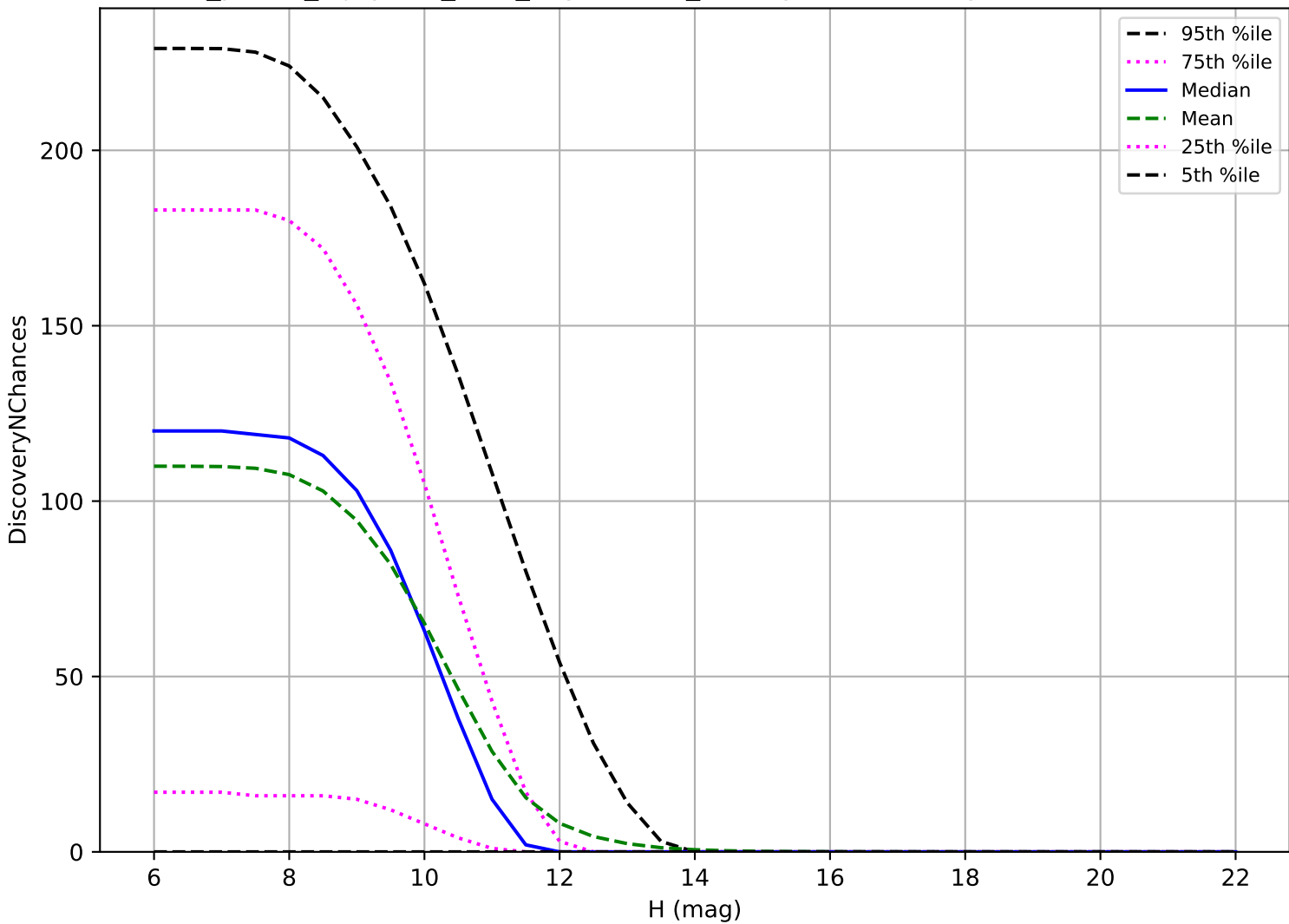
roll_pause_mjdp365_v3.4_10yrs: OCC_r20 3 pairs in 15 nights detection loss
