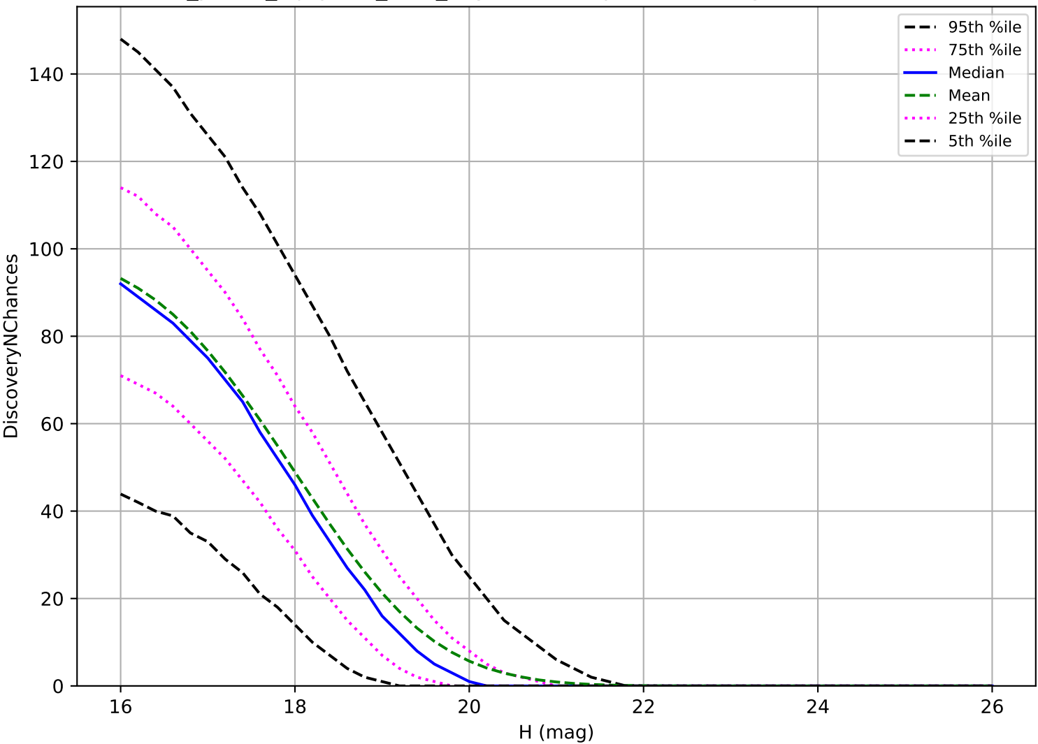
roll_pause_mjdp365_v3.4_10yrs: MBA 3 pairs in 15 nights detection loss
