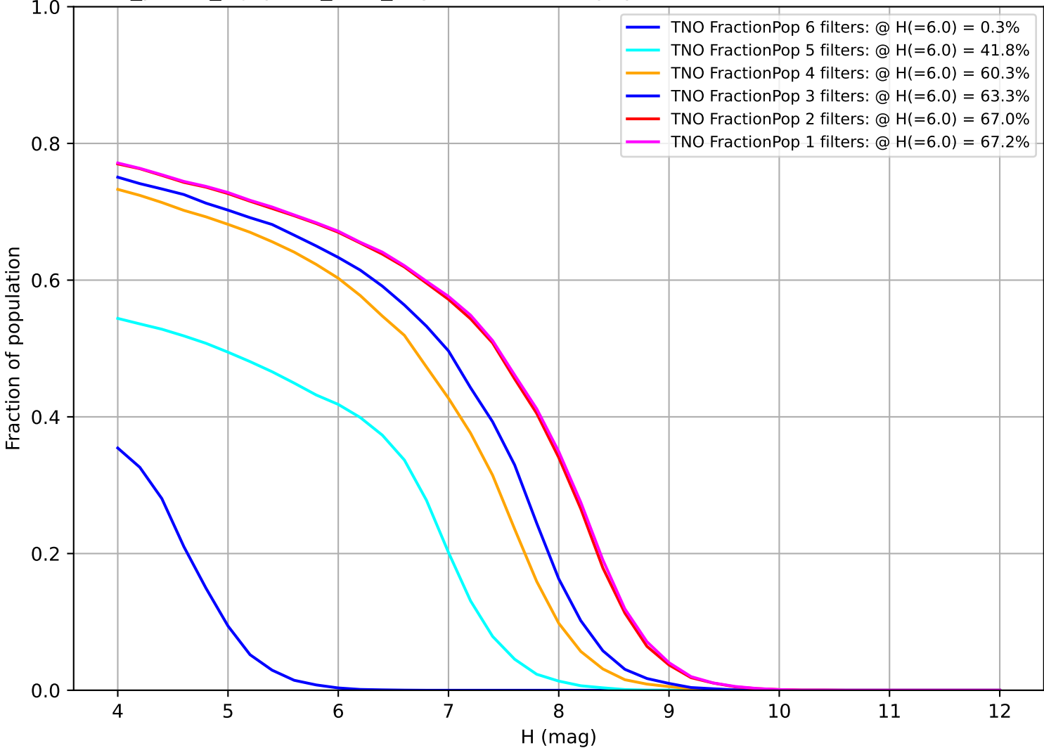
roll_pause_mjdp365_v3.4_10yrs: Fraction of population with colors in X filters TNO
