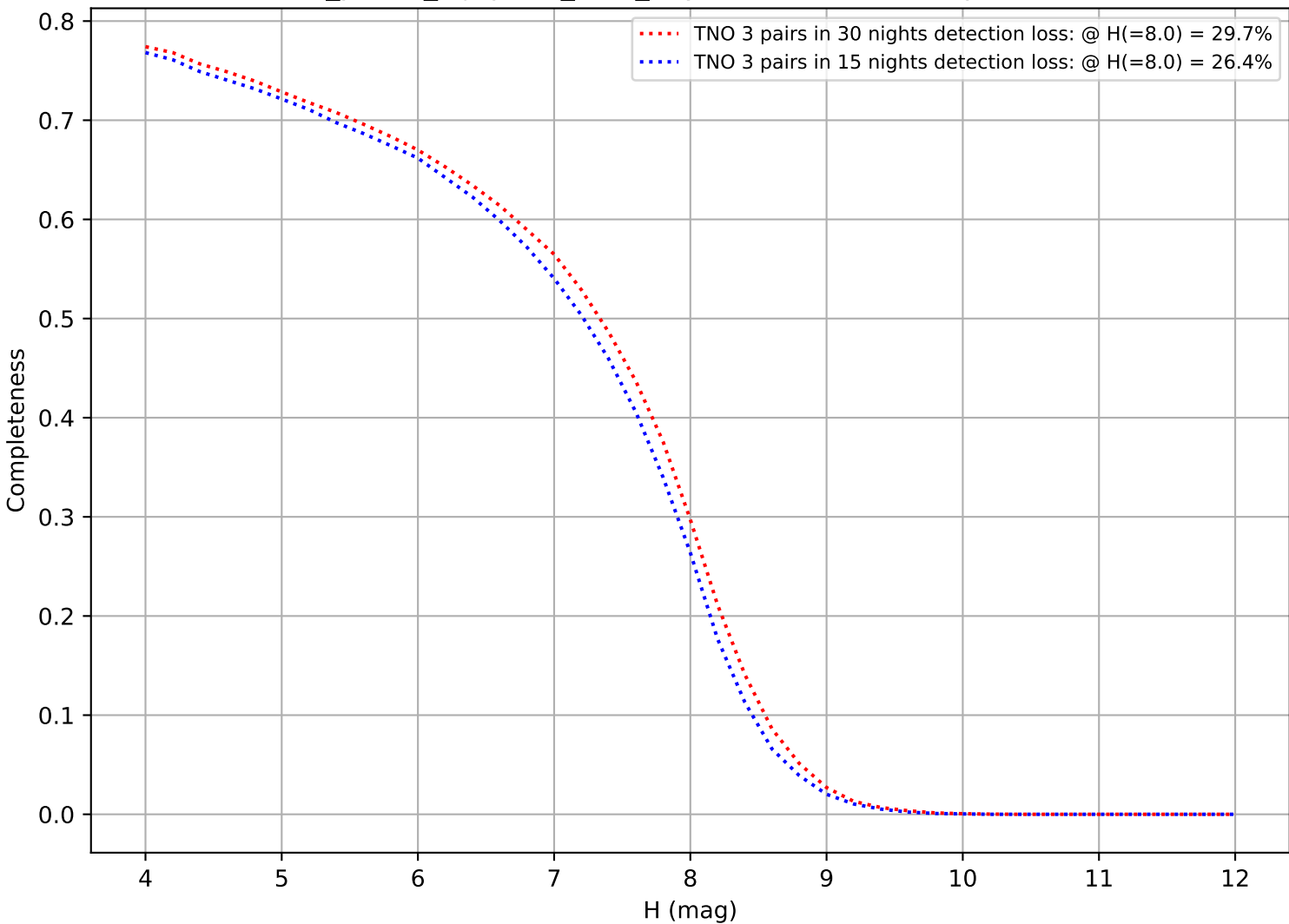
roll_pause_mjdp365_v3.4_10yrs: DifferentialCompleteness
