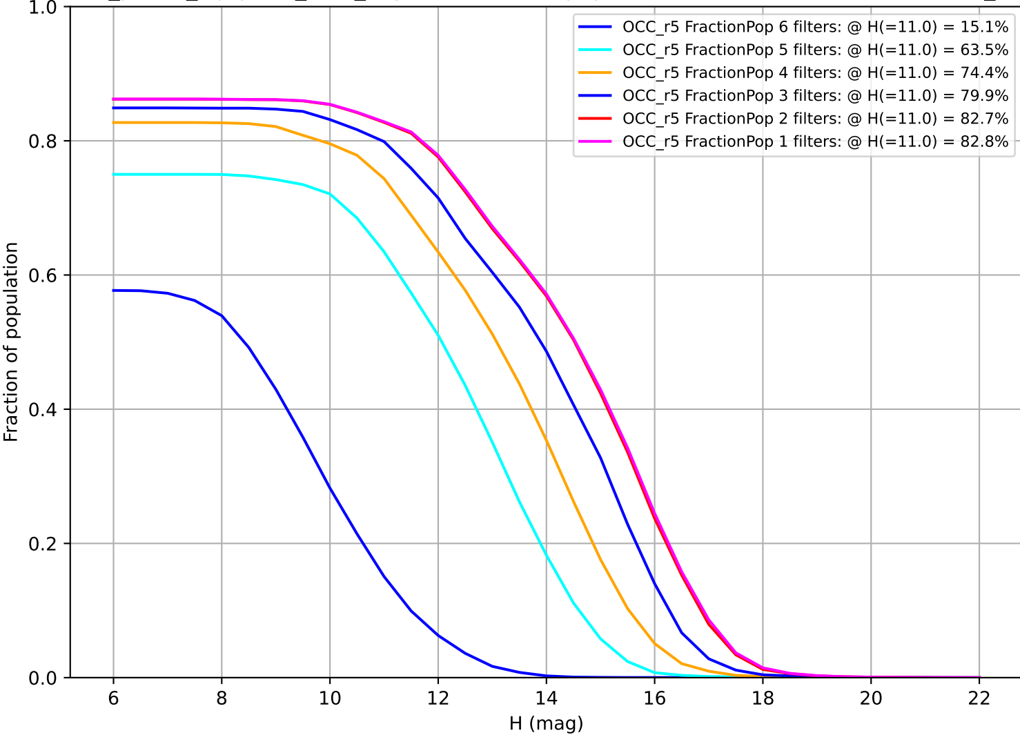
roll_pause_mjdp365_v3.4_10yrs: Fraction of population with colors in X filters OCC_r5
