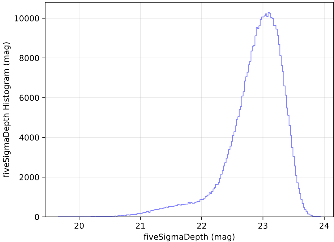
roll_pause_mjdp365_v3.4_10yrs z: fiveSigmaDepth Histogram
