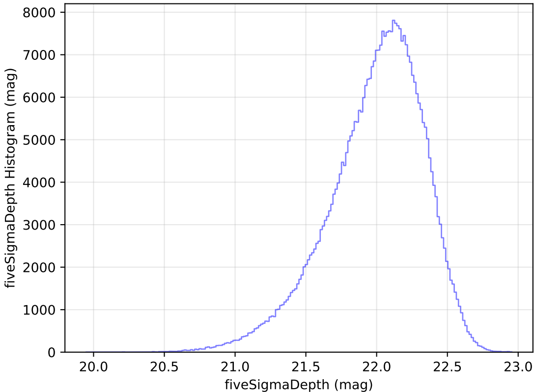
roll_pause_mjdp365_v3.4_10yrs y: fiveSigmaDepth Histogram
