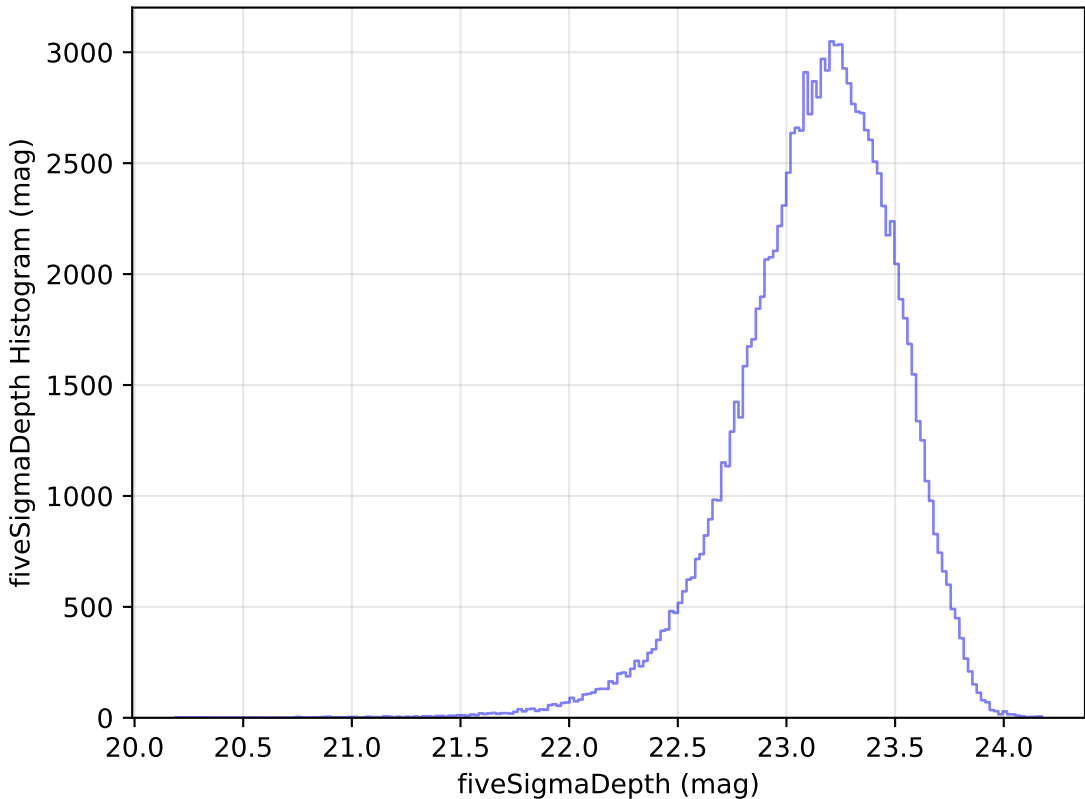
roll_pause_mjdp365_v3.4_10yrs u: fiveSigmaDepth Histogram
