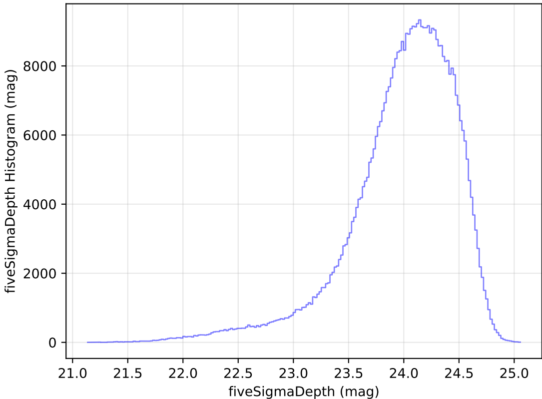
roll_pause_mjdp365_v3.4_10yrs r: fiveSigmaDepth Histogram
