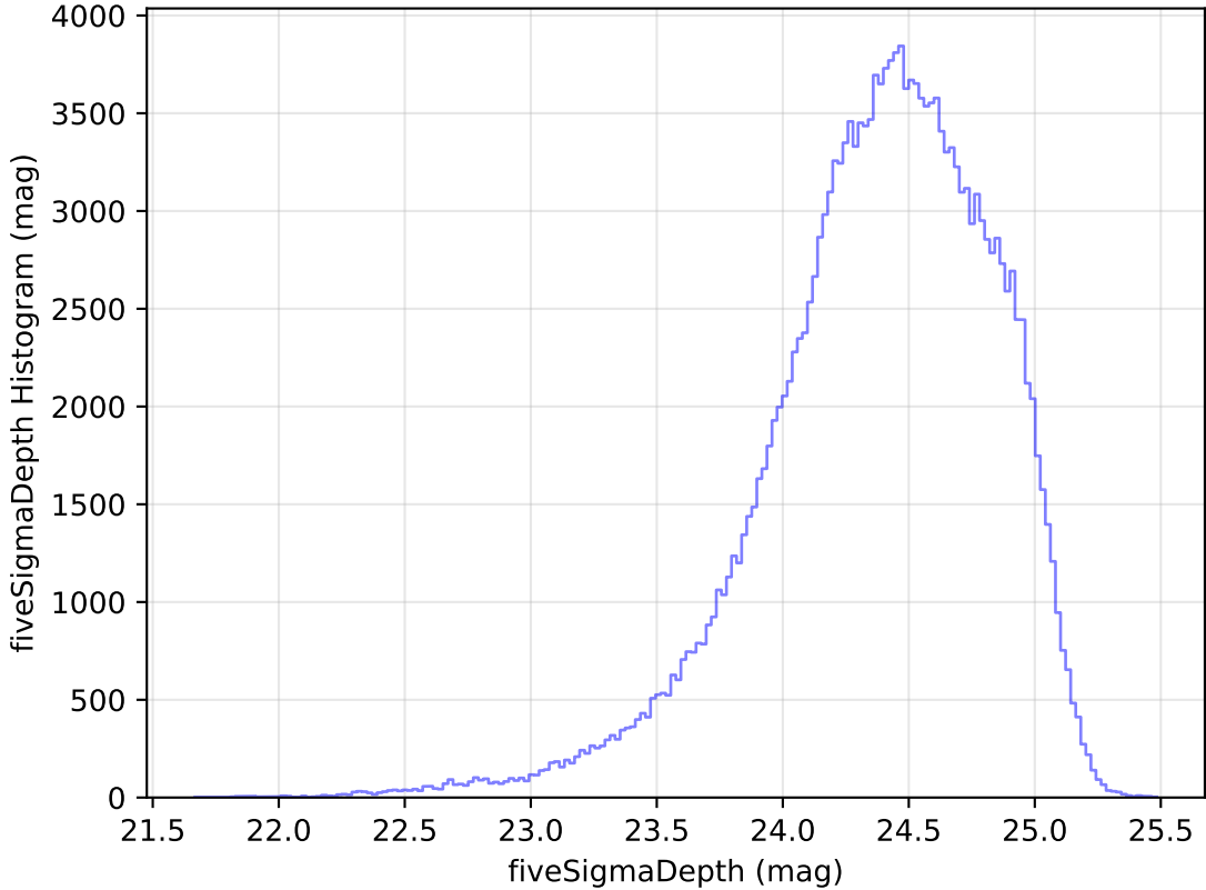
roll_pause_mjdp365_v3.4_10yrs g: fiveSigmaDepth Histogram
